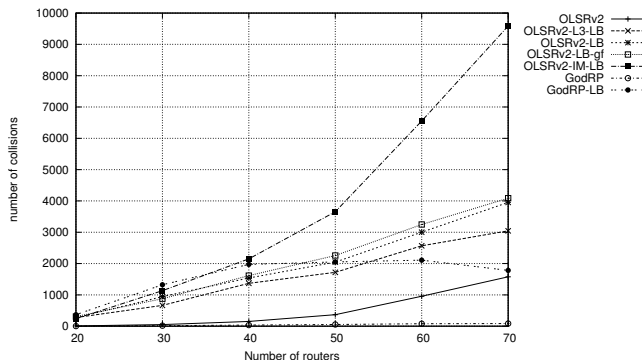
Figure 11. Collisions
