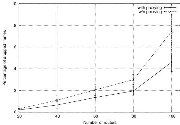
Figure 8. MAC frame drop ratio (90% confidence intervals)
