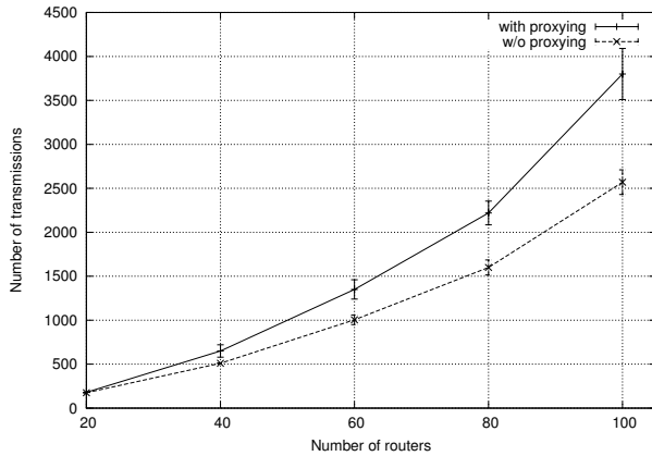
Figure 7. Total number of transmissions (90% confidence intervals)
